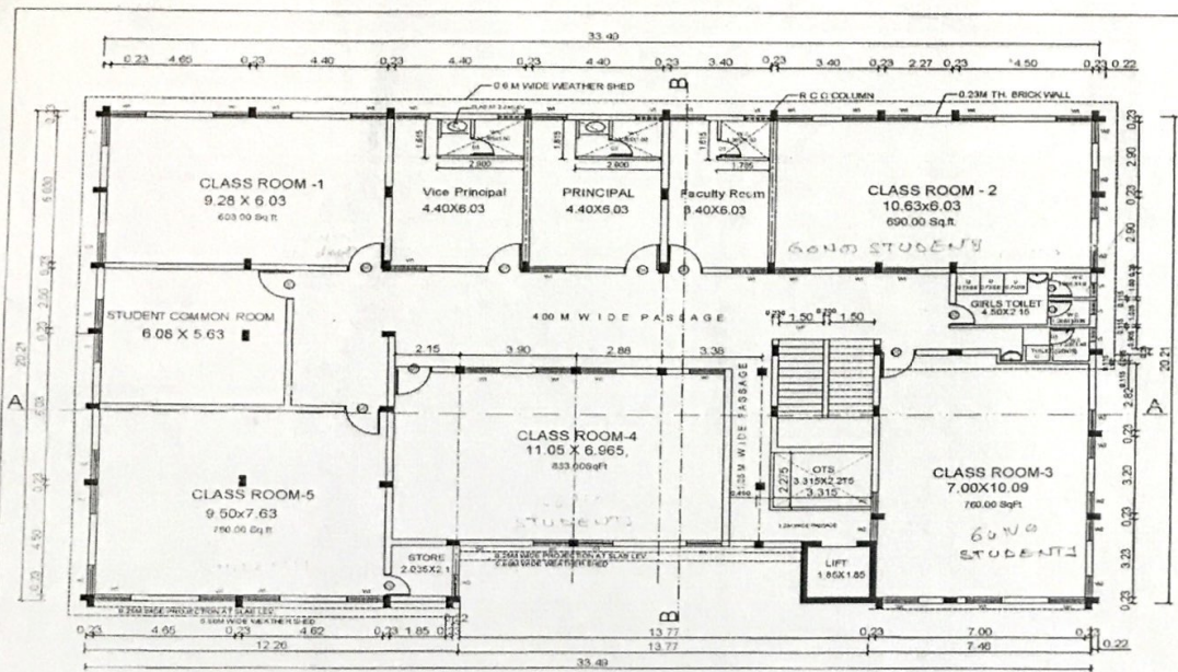
THIRD FLOOR PLAN FOR G.N.M. COURSE Area : 630.00 smt. SCALE: 1 CM = 1.0 M
