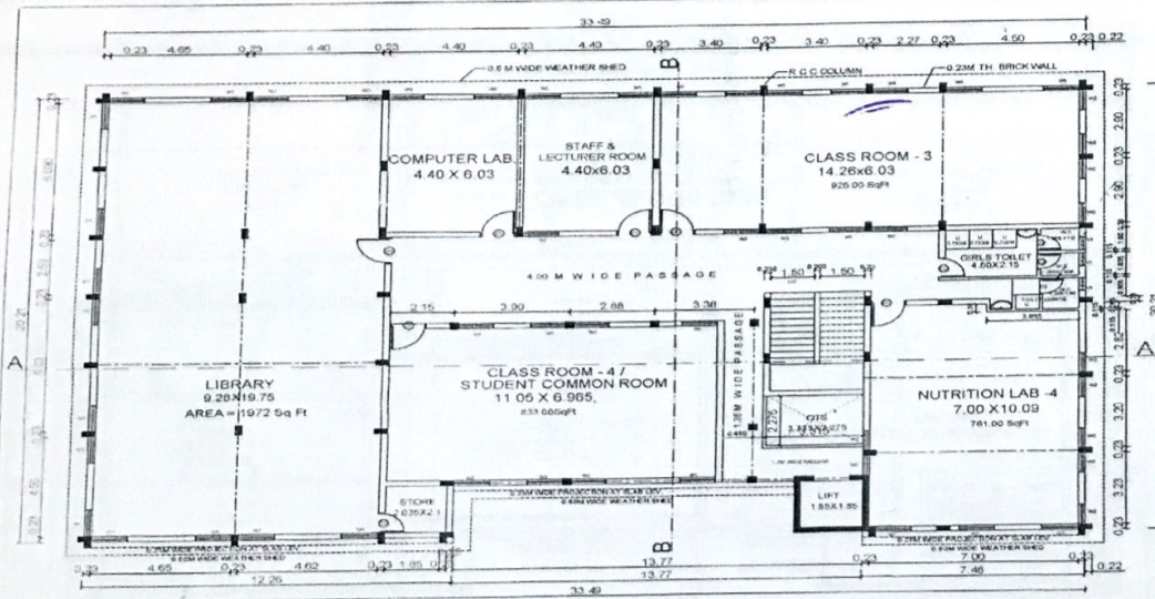
SECOND FLOOR PLAN Area : 630.00 smt SCALE: 1 CM = 1.0 M
